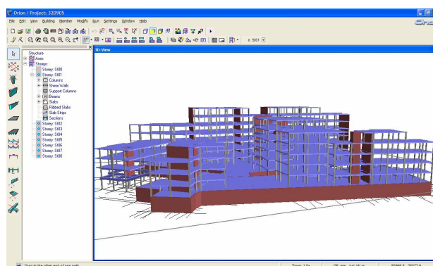
▶ PEP Group model in CSC Orion
