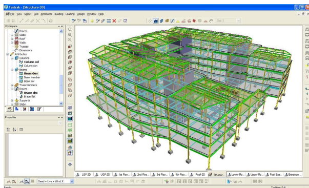
▶ PEP Group model in CSC Fastrak Building Designer
